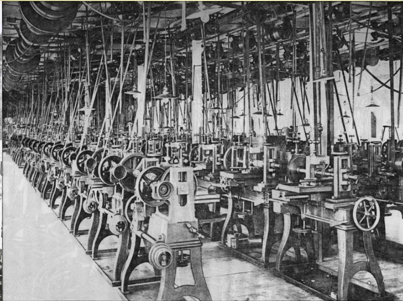
PRATT & WHITNEY LINCOLN MILLING MACHINES. U. S. ARMOY, SPRINGFIELD, MASS.
